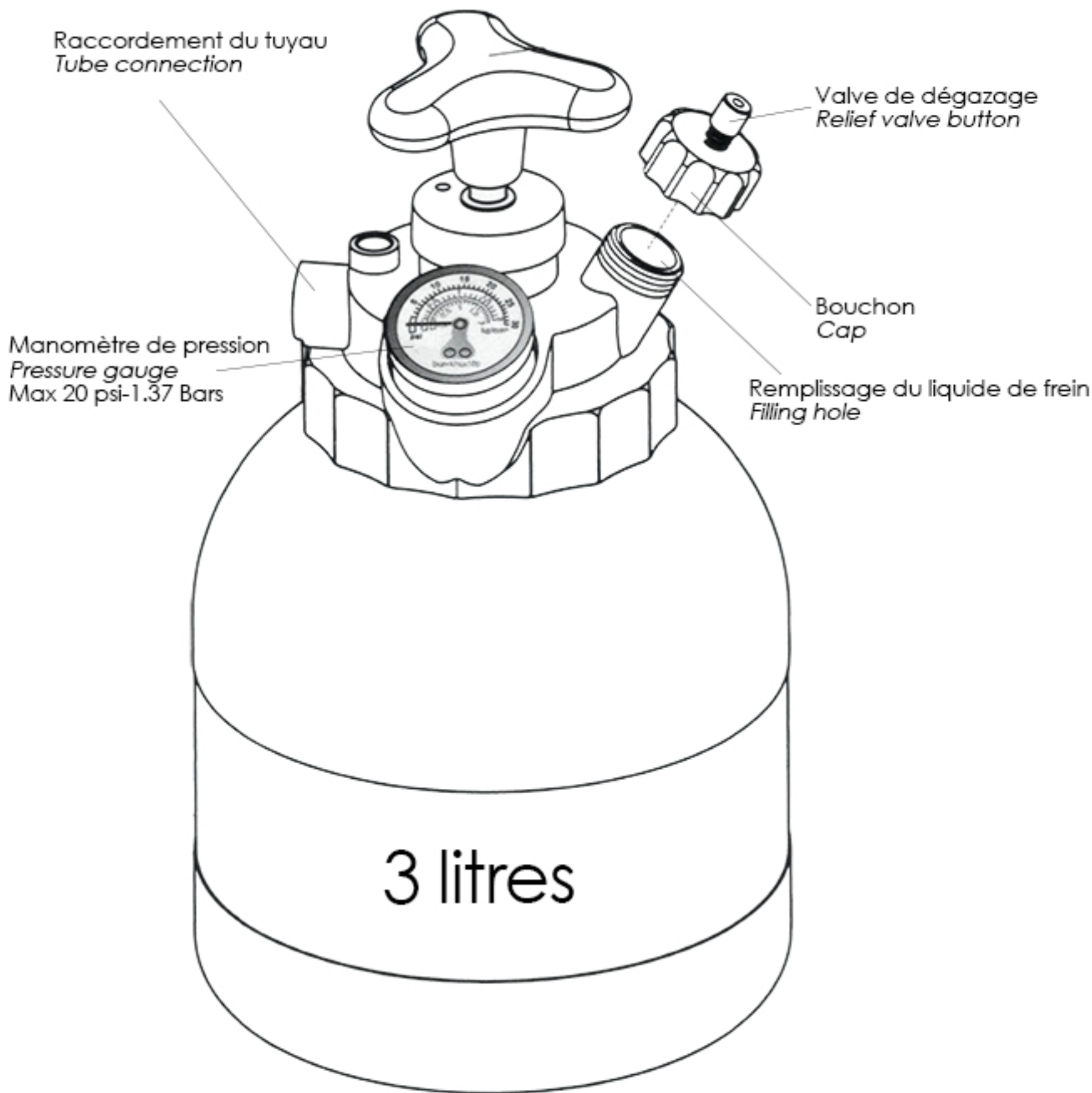
Raccorder le tuyau principal Firmly connect the main tube
